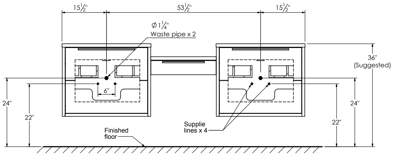
ROUGHING-IN DIMENSIONS
