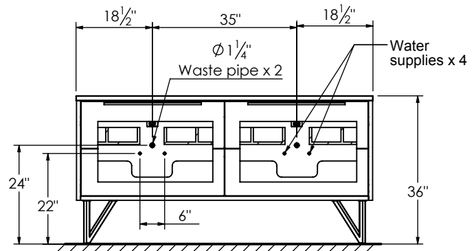
ROUGH PLUMBING
