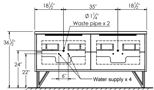
ROUGH PLUMBING
