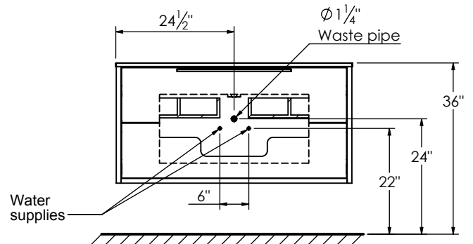
ROUGH PLUMBING
