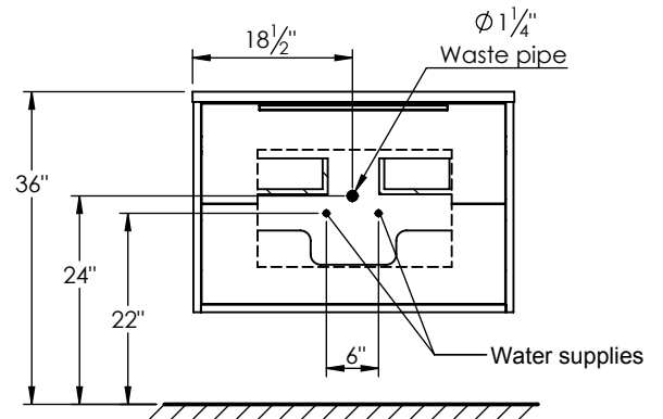
ROUGH PLUMBING
