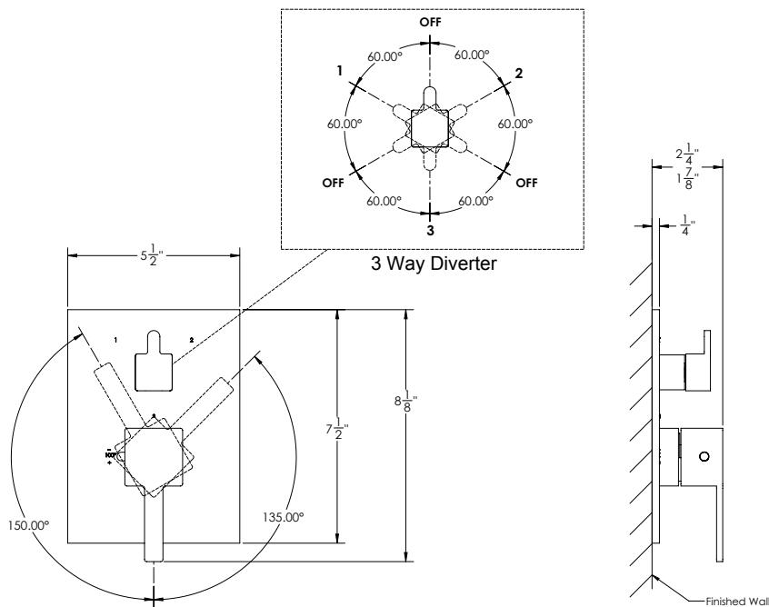
IS203-1-X Trim set
