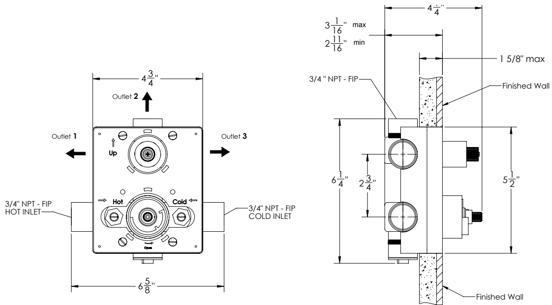
IS203 Rough valve
